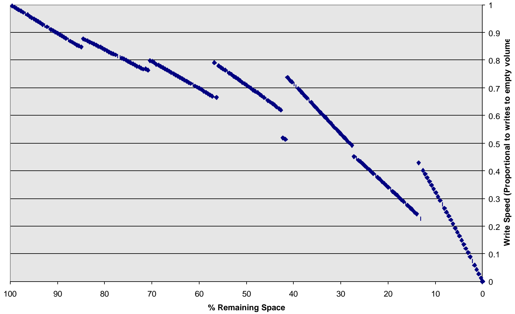
TargetFFS: Write Speed vs. Remaining Space
